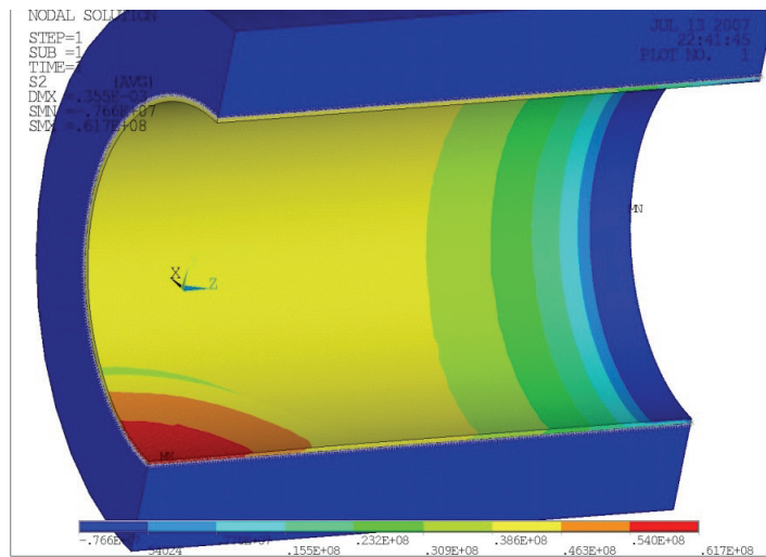
Fig. 22. Distribution of the stress \sigma_2 ( \sigma_t ) at \sigma_r|_{r=r_1} = p , \sigma_r^{(1)}|_{r=r_2} = -\sigma_r^{(2)}|_{r=r_2} , \sigma_\tau^{(1)}|_{r=r_2} = -\sigma_\tau^{(2)}|_{r=r_2} = f \sigma_{ii}^{(1)}|_{r=r_2} , u_x|_{r=r_3} = u_y|_{r=r_3} = 0
