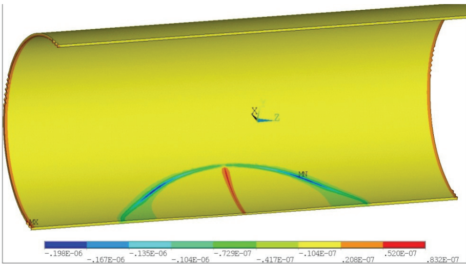
Fig. 34. Strains \epsilon_z at \sigma_r|_{r=r_1} = p, u_x|_{r=r_2} = u_y|_{r=r_2} = u_z|_{r=r_2} = 0
