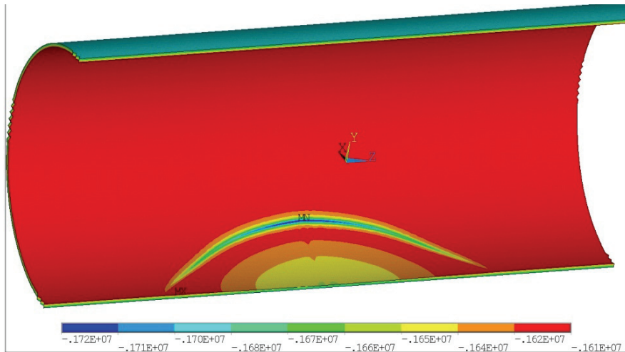
Fig. 19. Distribution of the stress \sigma_1(\sigma_i) at \sigma_r|_{r=r_1} = p, u_x|_{r=r_2} = u_y|_{r=r_2} = u_z|_{r=r_2} = 0
