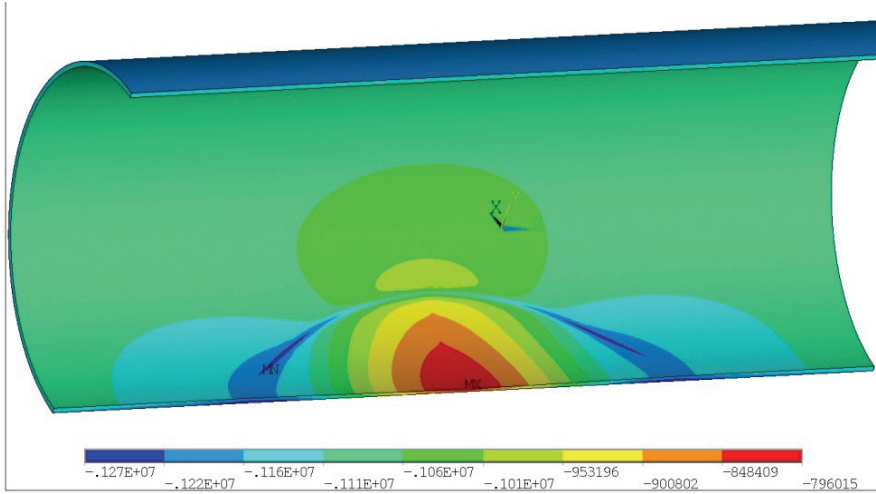
Fig. 18. Distribution of the stress \sigma_2(\sigma_i) at \sigma_r|_{r=r_1} = p, u_x|_{r=r_2} = u_y|_{r=r_2} = 0
