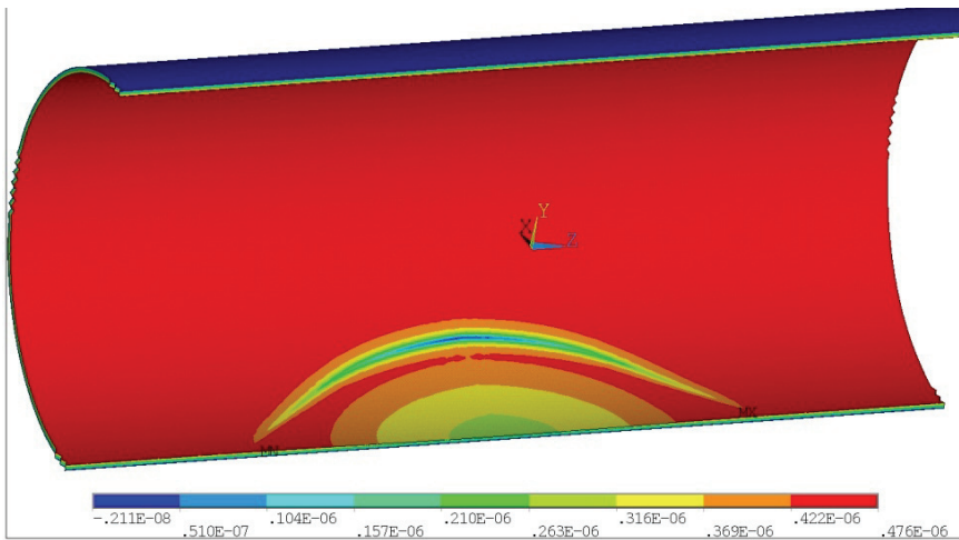
Fig. 30. Strains \epsilon_t at \sigma_r|_{r=r_1} = p, u_x|_{r=r_2} = u_y|_{r=r_2} = u_z|_{r=r_2} = 0
